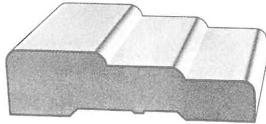
327 5/8 x 2-1/2
