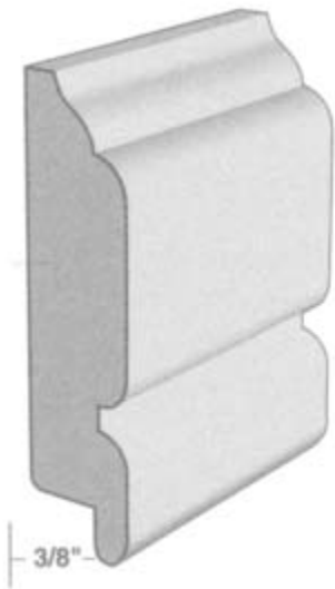
993 9/16 x 2-1/4
